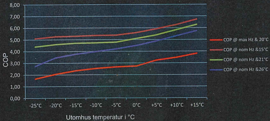
COP vs. utomhus temperatur MSZ-FH25VEHZ
