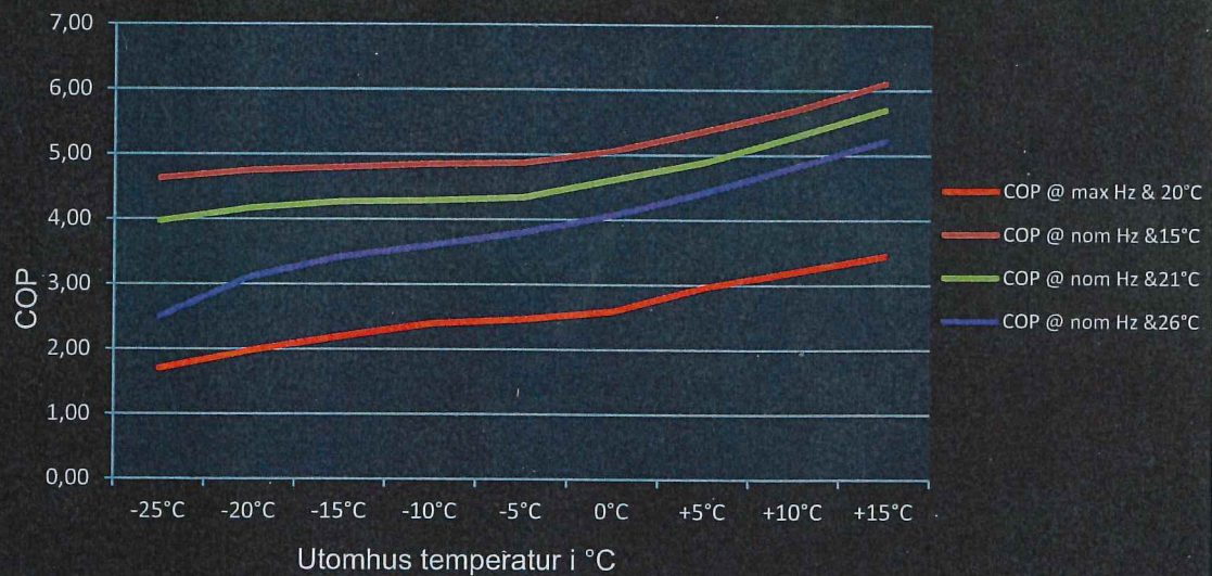
COP vs. utomhus temperatur MSZ-FH35VEHZ
